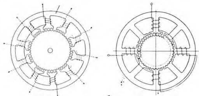
FIVE PHASE STATOR DESIGN
